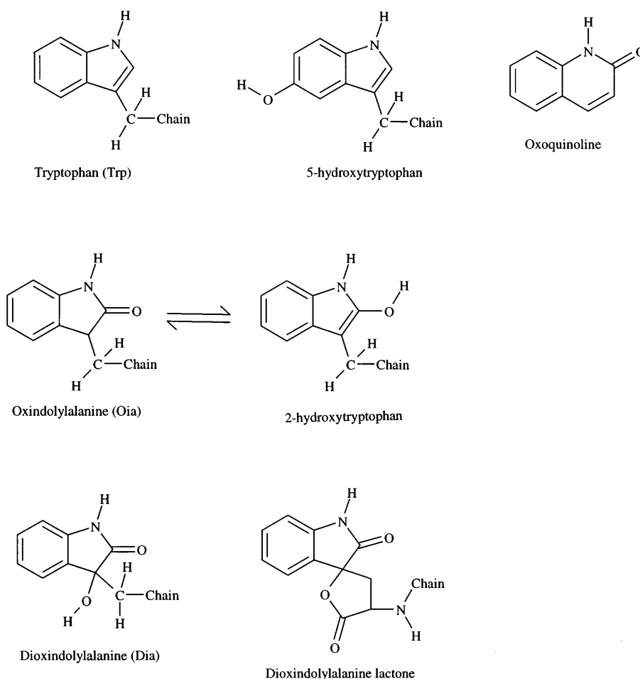
Scheme 1. Tryptophan and related (oxidation) products.
