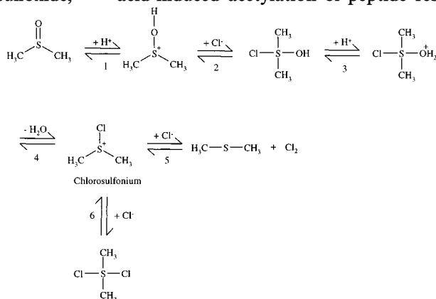
Scheme 3. Equilibria in water-containing DMSO–HCl mixtures (cf. Refs 25 and 27).
