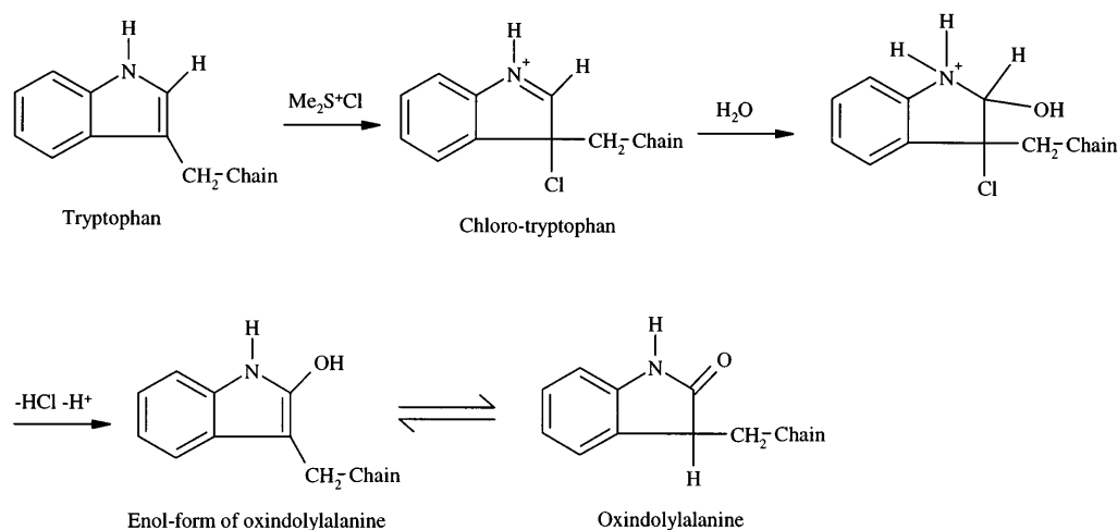
Scheme 2. Reaction scheme of tryptophan oxidation in DMSO–HCl–HAc (cf. Ref. 15).
