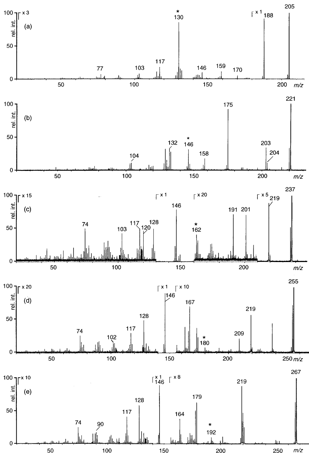
Figure 1. FAB-CID mass spectra of ions observed when Trp is treated with DMSO-HCl-HAc mixtures. (a) m/z 205; (b) m/z 221; (c) m/z 237; (d) m/z 255; (e) m/z 267. Complete side-chain ions are indicated by asterisks.
