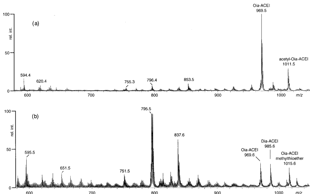
Figure 3. FAB mass spectra of ACEI treated in an open tube for 1 h with DMSO–HCl–HAc mixtures containing (a) 3.75 and (b) 5.5 M HCl.
