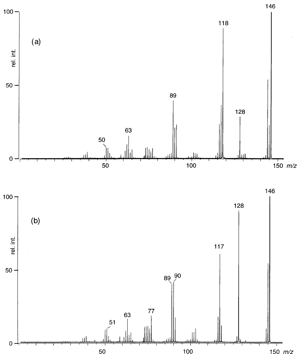
Figure 2. FAB-CID mass spectra of the fragment ion at m/z 146 of (a) Oia and (b) Dia.
