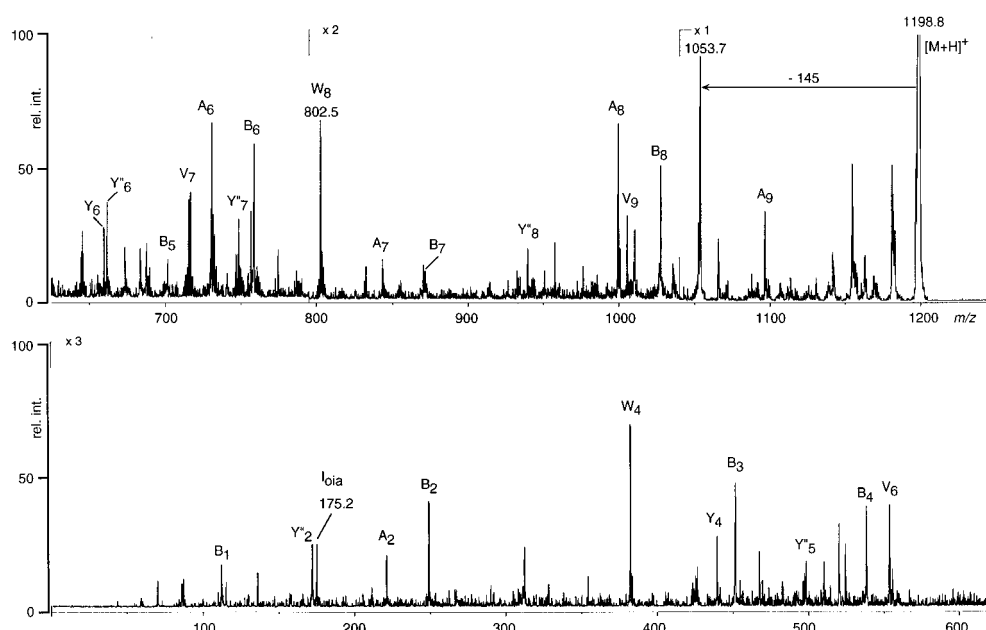
Figure 4. FAB-CID mass spectrum of Oia-containing luteinizing hormone-releasing hormone (pyroE-H-X-S-Y-G-L-R-P-G-NH 2 , in which X is Oia). Characteristic mass differences of Oia-containing peptides are indicated.
